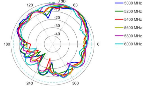
Elevation: 5000 – 6000 MHz
