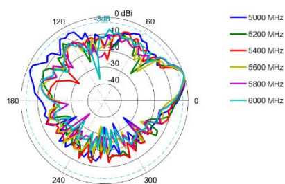
Elevation: 5000 – 6000 MHz
